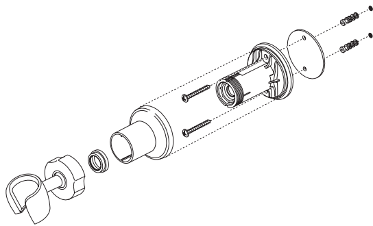
U4005-PK▲ Mounting Bracket Consola de montaje Support
